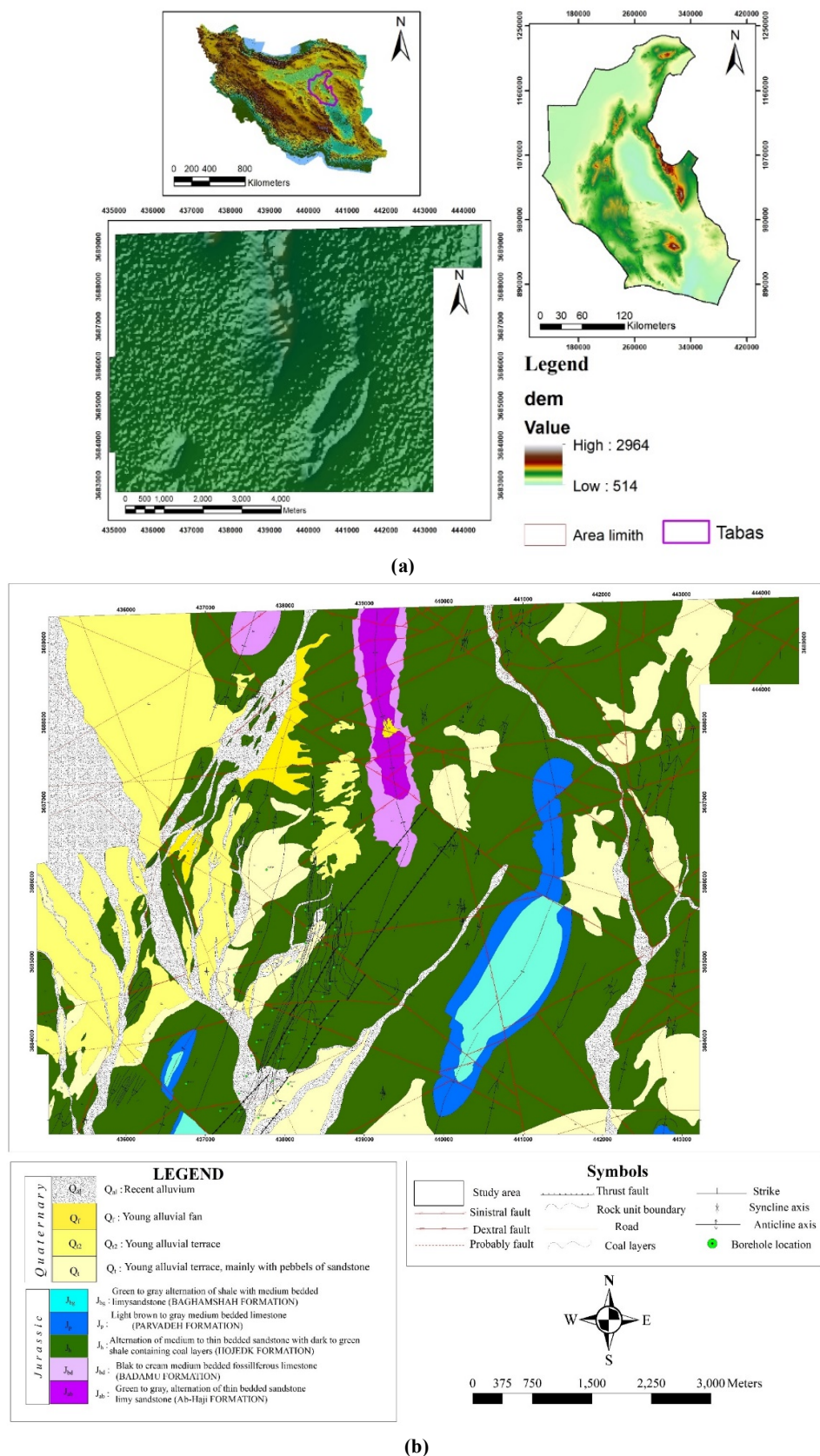
Figure 1. a- Geology setting (modified after [70]) b- Geology map of North Kochakali deposit (modified after [71]).
