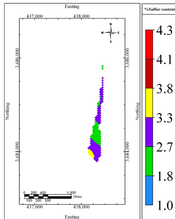
Figure 13. Sulfur plan map in K7 seam at 1100 meters.
