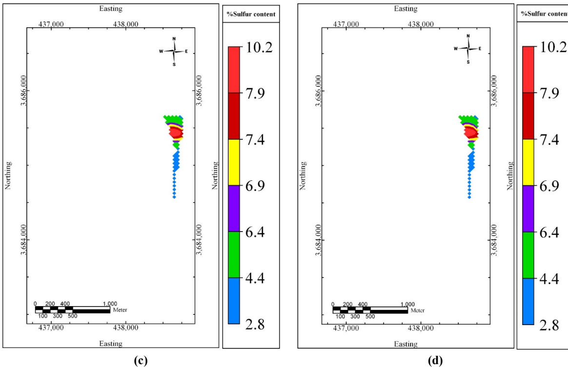
Figure 9. Sulfur plan map in K1 seam (c- at 900 meters and d- at 1000 meters).
