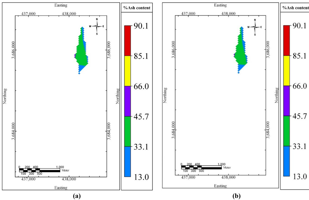
Figure 17. Ash plan map in K7 seam (a- at 755 meters and b- at 800 meters).
