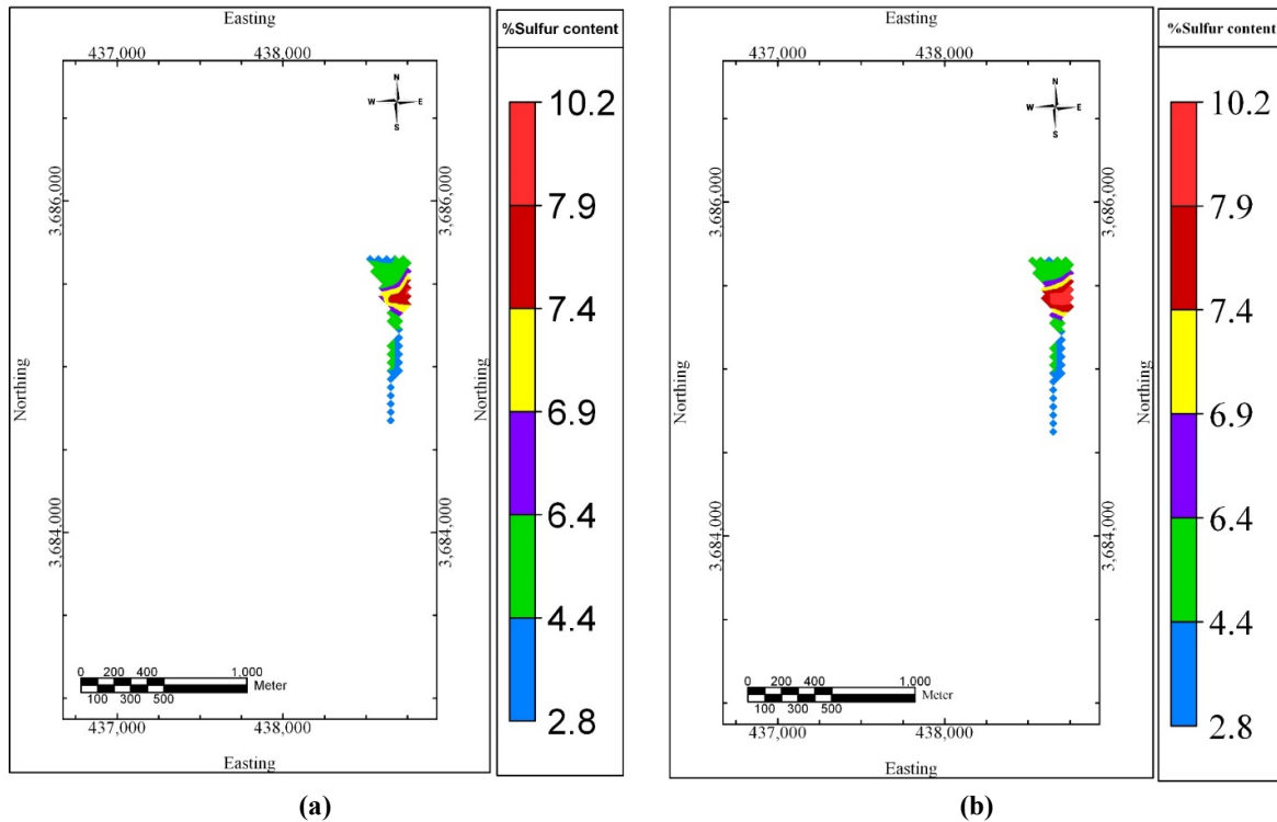
Figure 8. Sulfur plan map in K1 seam (a- at 755 meters and b- at 800 meters).
