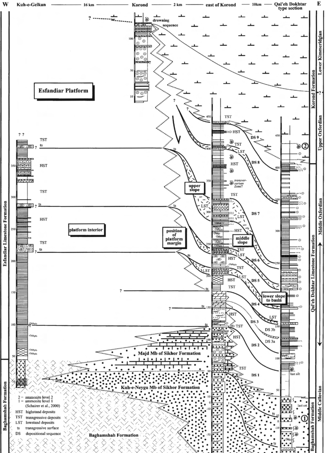
Fig. 9. Platform-basin correlation based on four sections (simplified after Figs 4-7). Note bioclastic lowstand wedges on the middle slope and the bundling of platform top-derived calciturbidites on the lower slope (interpreted as highstand shedding) as well as the spreading of the basal Korond Formation over the platform top during the Late Oxfordian to Early Kimmeridgian (drowning). For key of symbols see Fig. 4.
