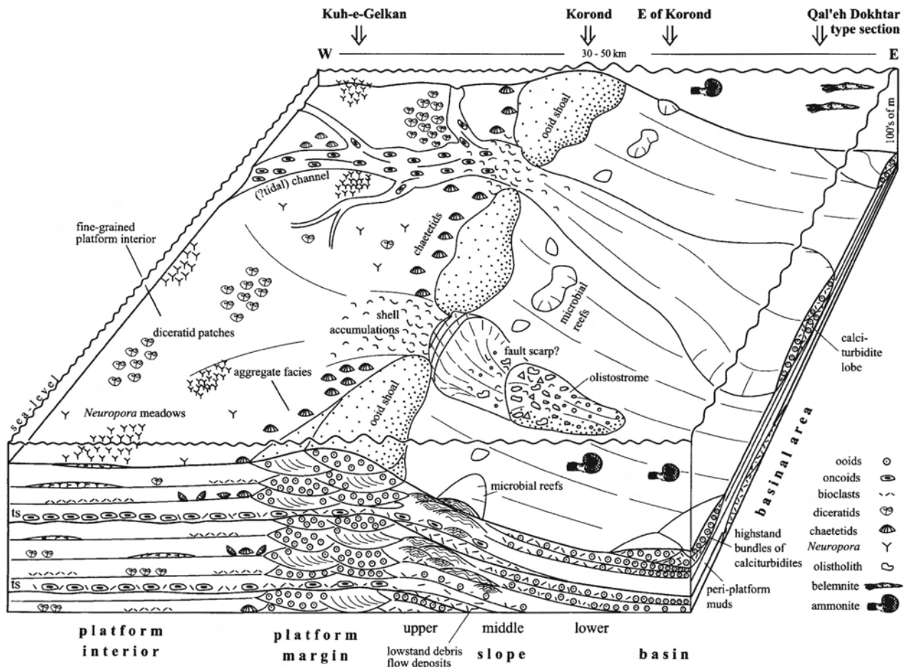
Fig. 10. Synoptic facies model of the eastern margin of the Esfandiar Platform based on sections between Esfak and Majd (see Fig. 2).
